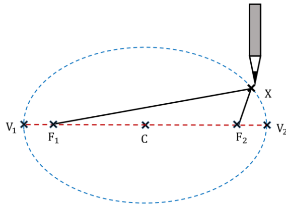
FIGURE 2: Ellipse by tracing points where the sum of distance from foci is a constant.
