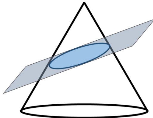
FIGURE 3: Ellipse by intersecting a cone with an inclined plane.
